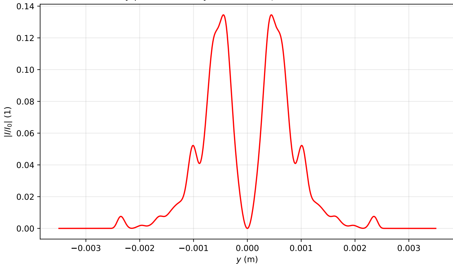
Intensity profile I(x=0, y, z=3.503)/I_0 , \text{Pin}=7.0\text{Pcr} , artificial time
